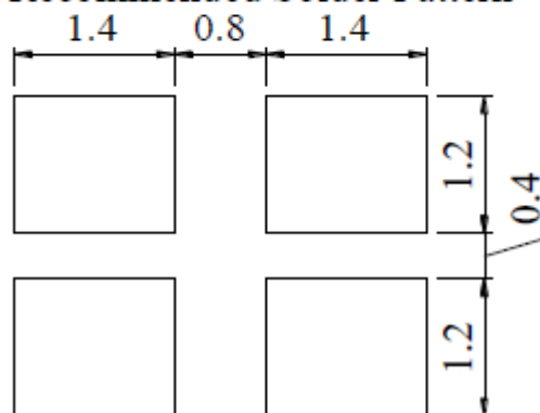
Recommended Solder Pattern
