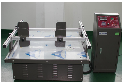
汽车振动模拟运输仪 Automobile vibration simulation transporter
